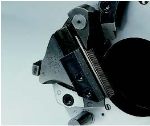
Chaser holder with chaser
